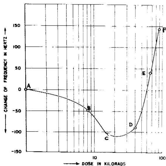
Fig. 2 Steady frequency offsets of a natural AT-cut quartz crystal irradiated in stages A, B,.....E. Accumulated doses at B = 8,000 Rads, at C = 16,000 Rads, at D = 40,000 Rads, at E = 64,000 Rads and at F = 88,000 Rads.
