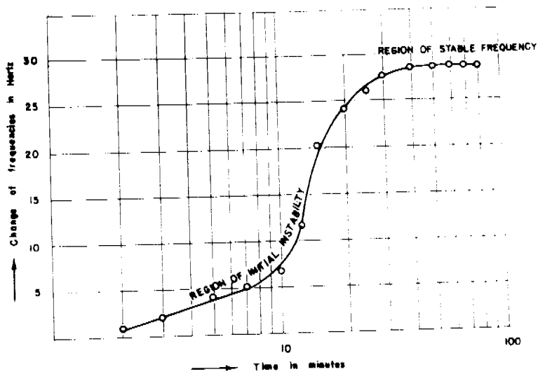
Fig-11 Frequency behavior of a natural AT-cut (1.87 MHz) quartz crystal with time after irradiation with fast neutrons with accumulated dose of 2 \times 10^{12} nvt using ^{241}\text{Am} - \text{Be} .
