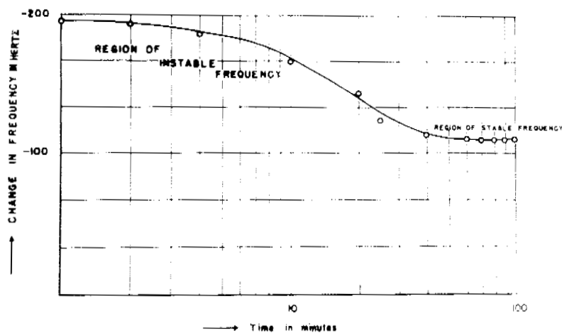
Fig.8 Frequency behavior of a natural AT-cut quartz crystal (1.87 MHz) irradiated by fast neutrons with a dose of 16 \times 10^{10} nvt and allowed to oscillate.
